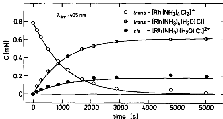
Fig. 2. Photolysis of a 0.79 mM trans -dichlorotetraamminerhodium(III) aqueous solution, cf. Fig. 1 (ref. 27).
