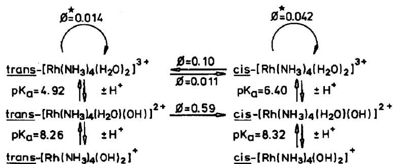
Fig. 4. Aqueous solution photochemistry of cis - and trans -diaqua-tetraamminerhodium(III) and conjugate bases. \Phi^* are quantum yields for stereoretentive water exchange (1 M perchlorate, ref. 19 and 33).
