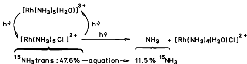
Fig. 8. Photolysis of chloropentaamminerhodium(III) in 0.5 M Cl^- gives eventually cis/trans -aquachlorotetraamminerhodium(III) plus cis/trans -dichlorotetraamminerhodium(III).
