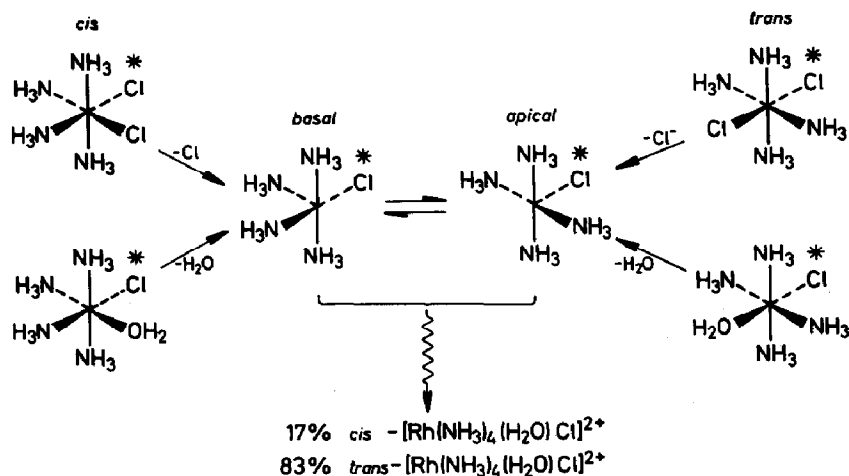
Fig. 3. Excited state reactions of cis - and trans -aquachlorotetraamminerhodium(III) and cis - and trans -dichlorotetraamminerhodium(III) within a limiting dissociative model. The basal - and apical excited state isomers can rearrange to each other in competition with deactivation to the ground state (ref. 27).
